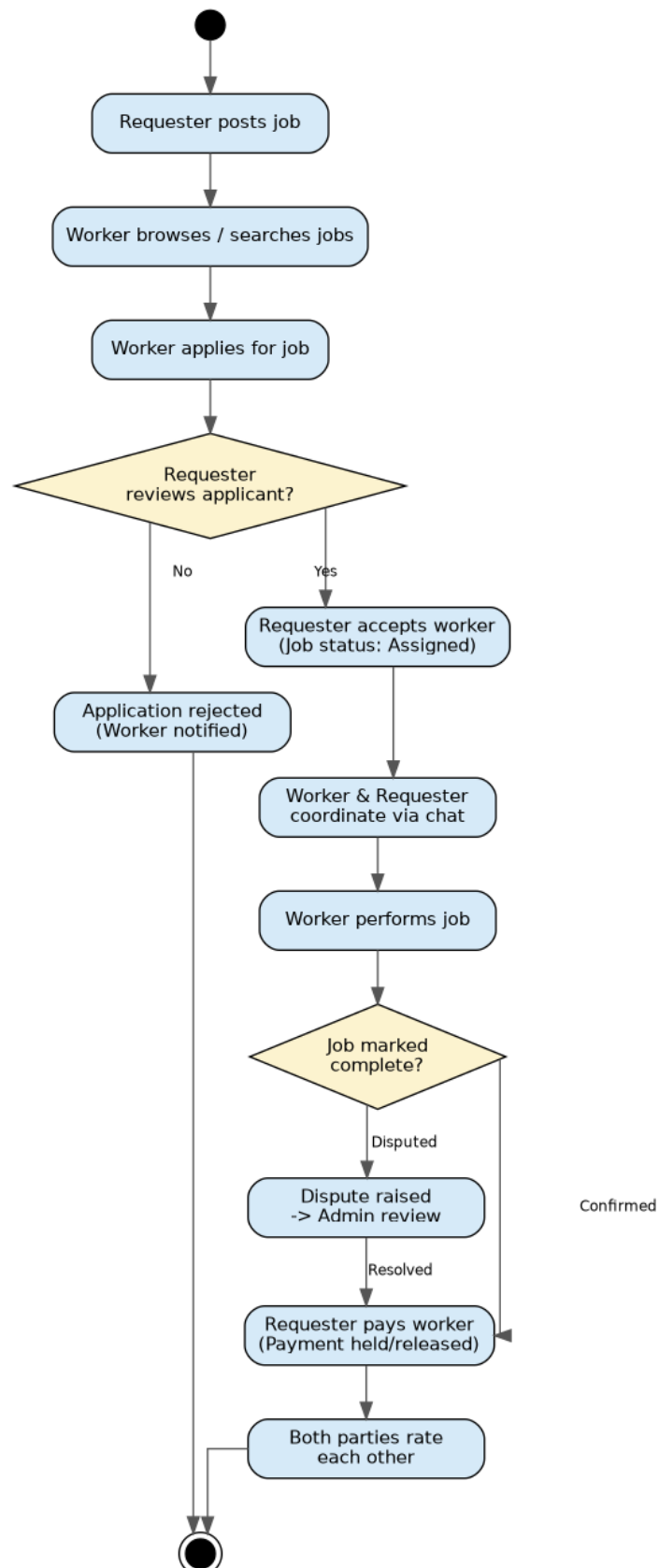
Figure 2 — Job Lifecycle Activity Diagram
